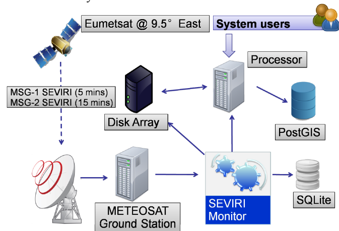
Figure 1. Fire monitoring service architecture of NOA
